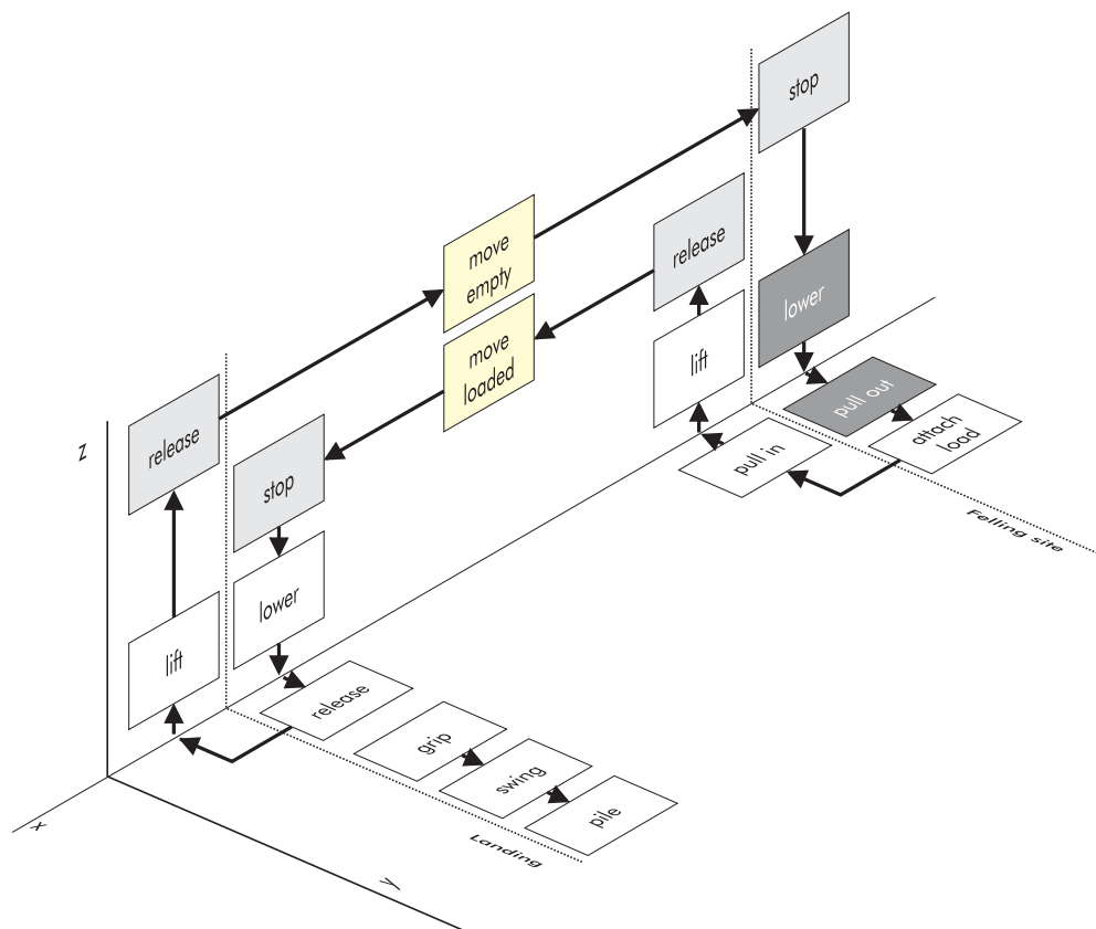
Fig 1: Technical functions of a cable yarding system. There are four functional groups: (1) transportation (x-axis), hoisting (z-axis), skidding (y-axis), and handling (y-axis).
